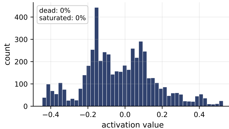
L4 (20 neurons)
