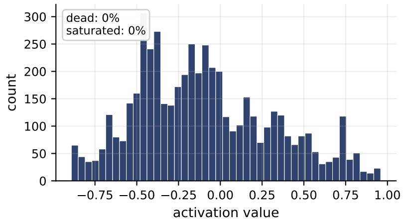
L3 (20 neurons)
