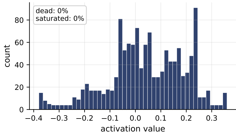
L3 (20 neurons)
