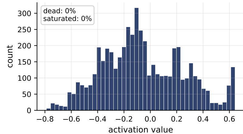
L5 (20 neurons)
