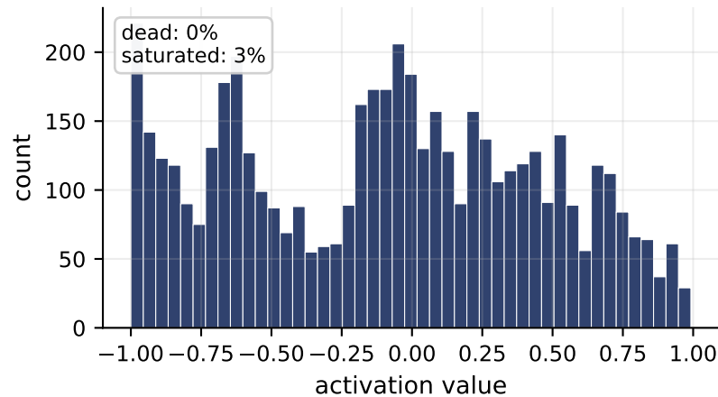
L4 (20 neurons)
